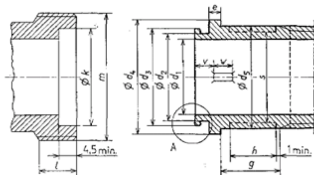
Figure 1: valve part
