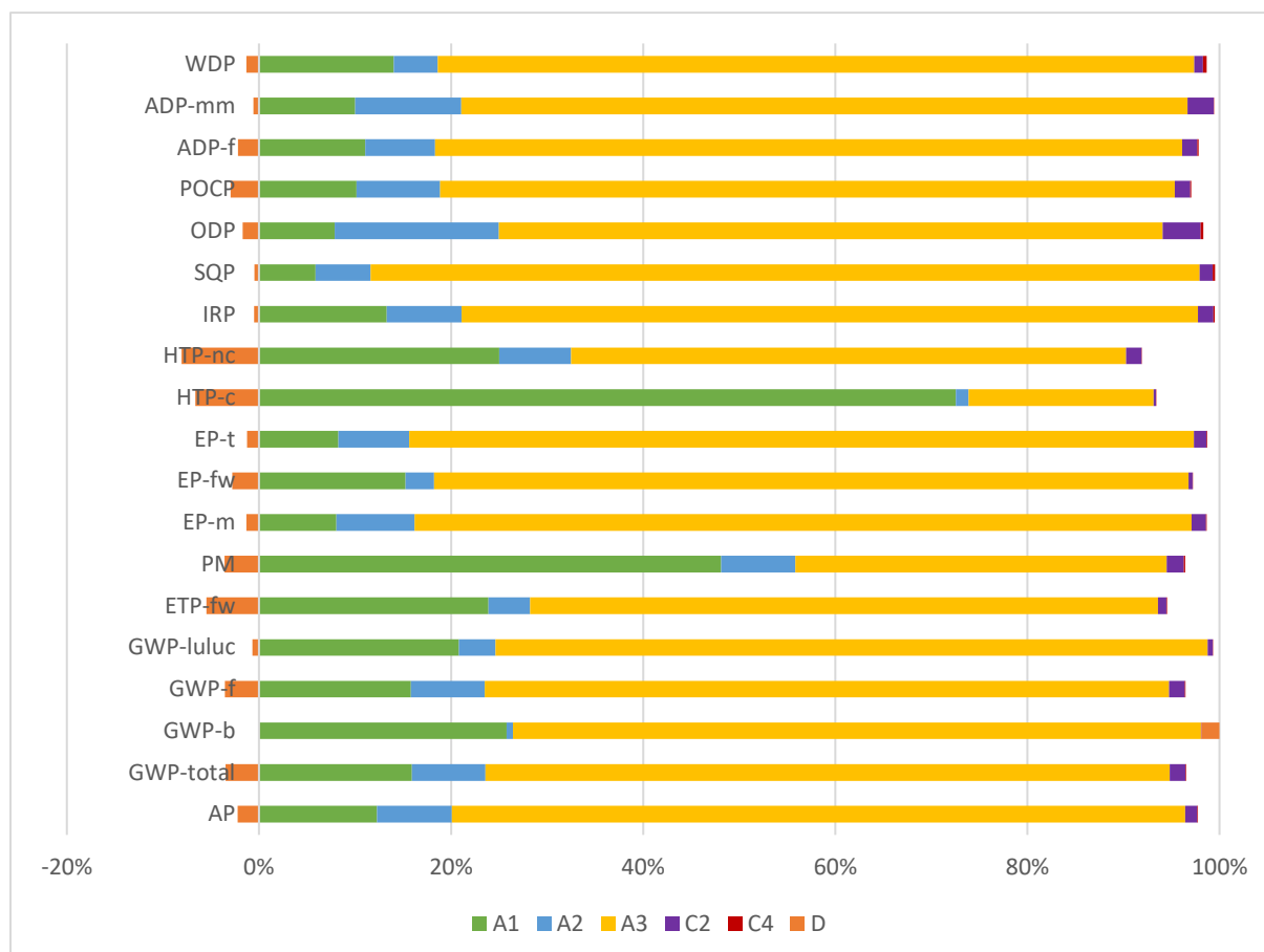
Figure 1 : Shares of the product life cycle phases in the environmental impact categories for wire rod
