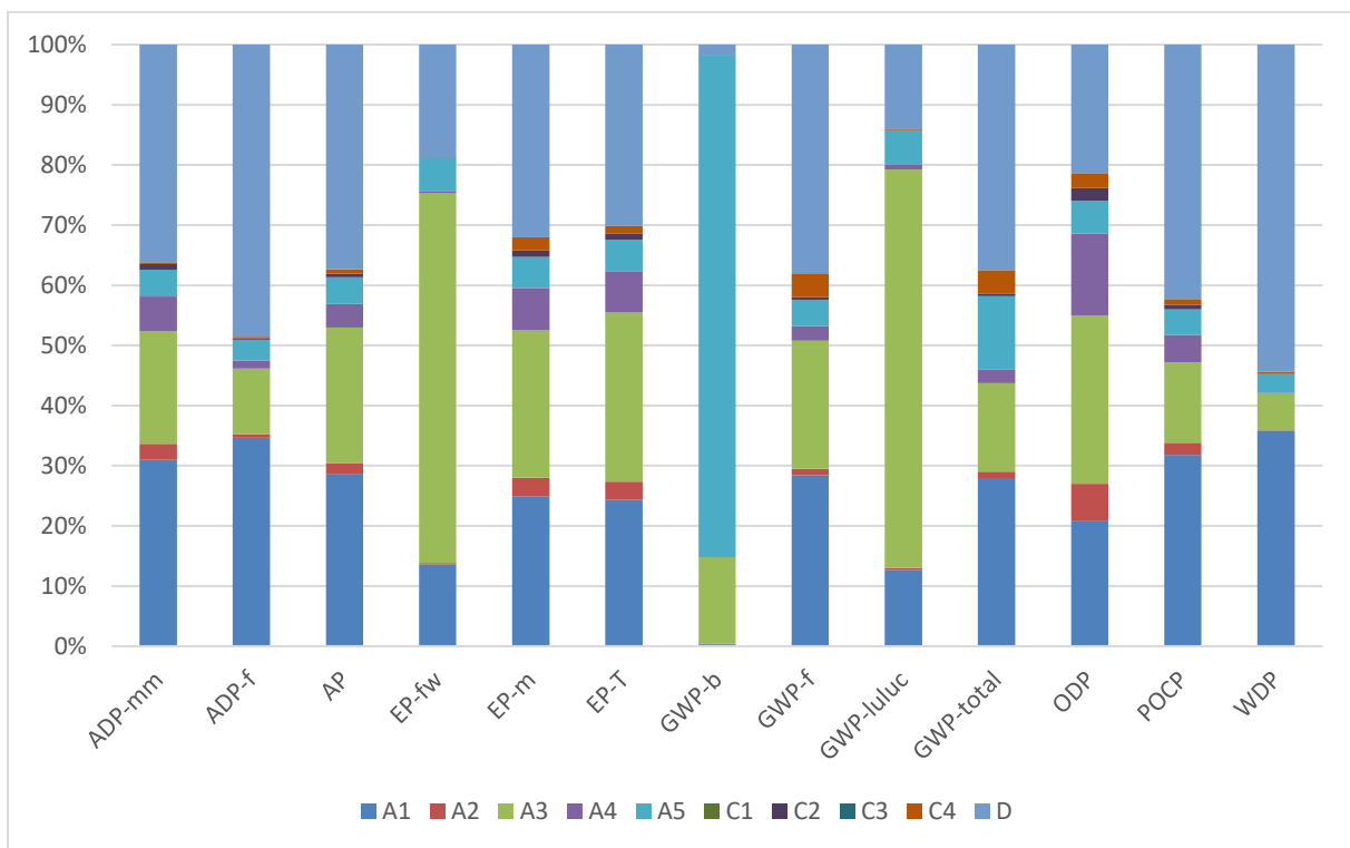
Figure 2: AQUAZIP ECO-LAMINA 2D - Impact of the individual modules on the environmental core indicators
