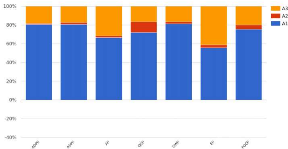
Graphic 1. Contribution by stages of composition Laminar (4+4).1 // 16 // Laminar (4+4).1
